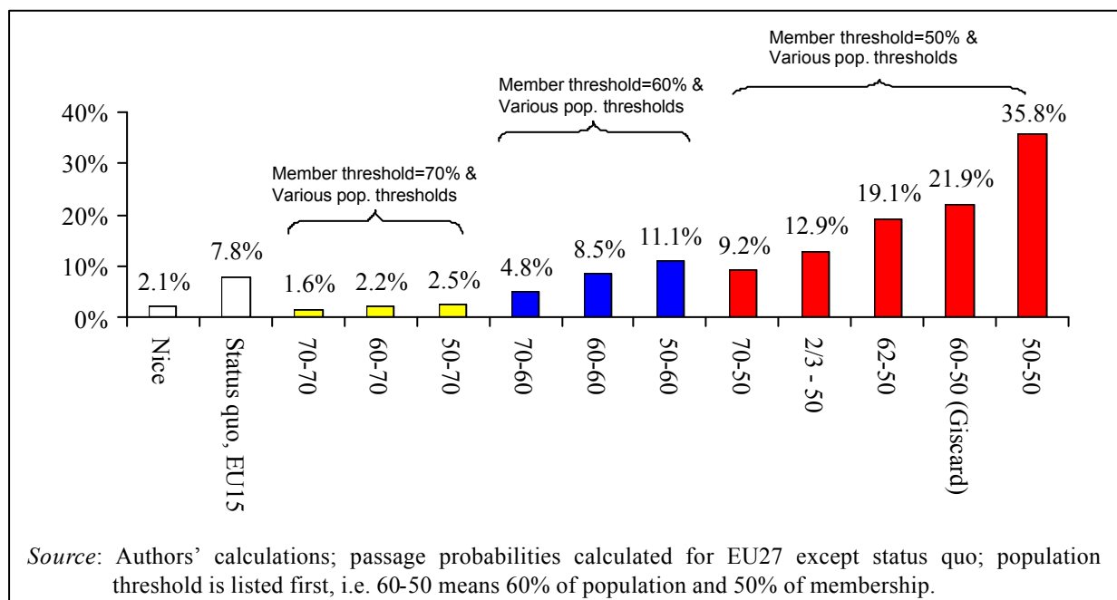
Figure 3. Passage probabilities, 11 different dual-majority schemes
