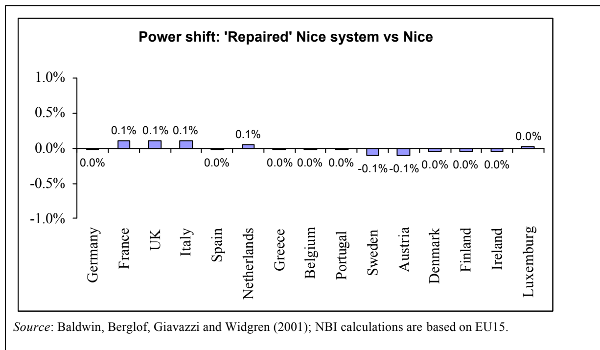
Figure 7. Power effects of 'repairing' the Nice system
