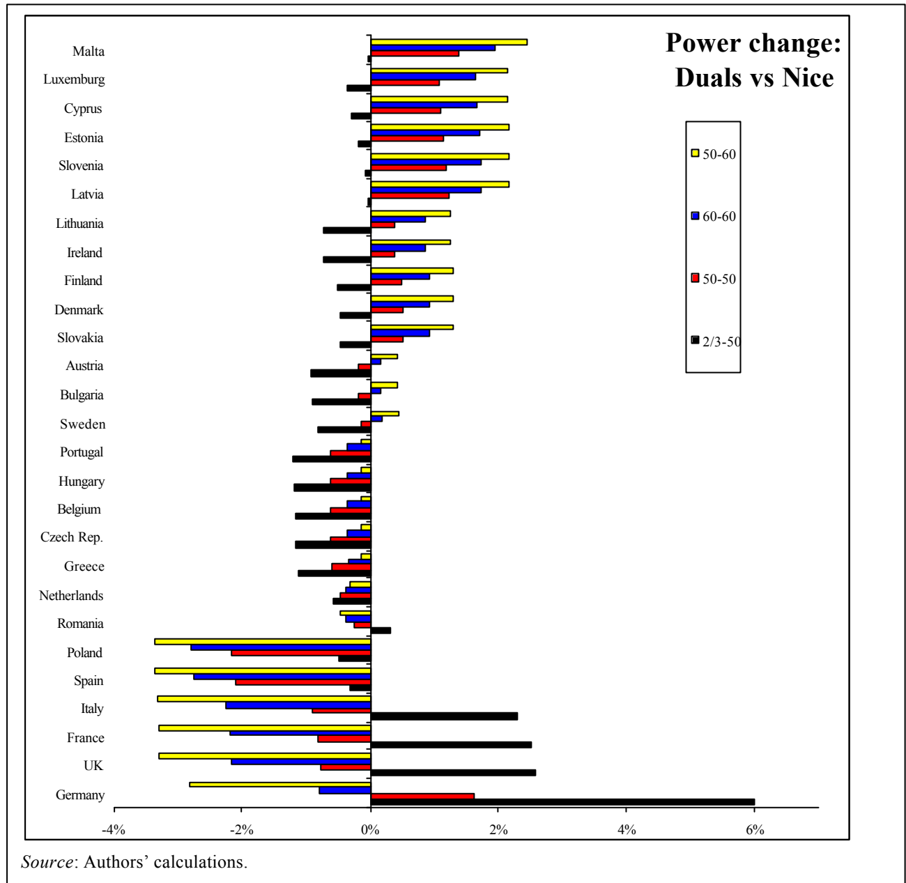
Figure 5. Power changes: various dual majority schemes vs. Nice
